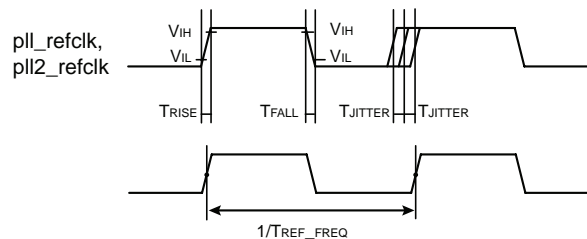
Figure 3-33 PLL timing diagram
