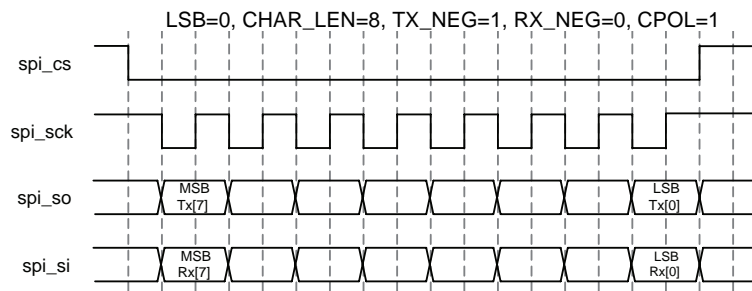
Figure 3-7 SPI timing 4
