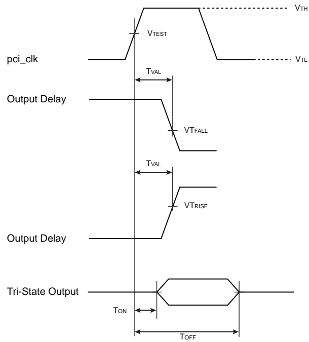
Figure 3-21 PCI output timing diagram
