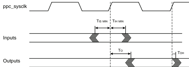
Figure 3-32 PowerPC timing
