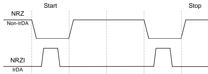
Figure 3-2 IrDA pulse
