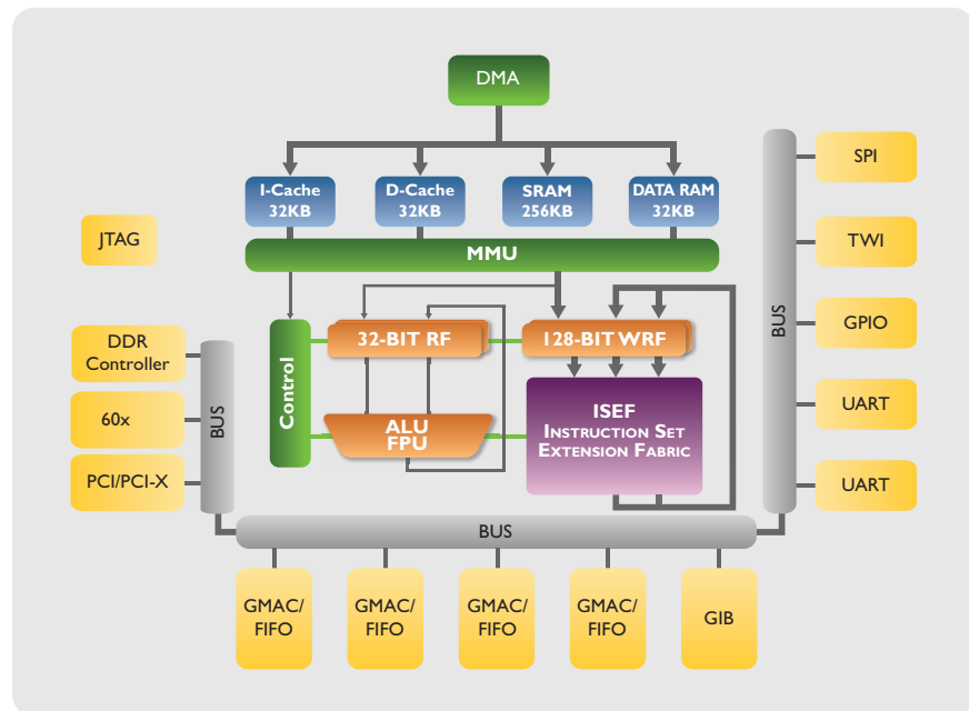
Figure 1 S5620 Block Diagram
