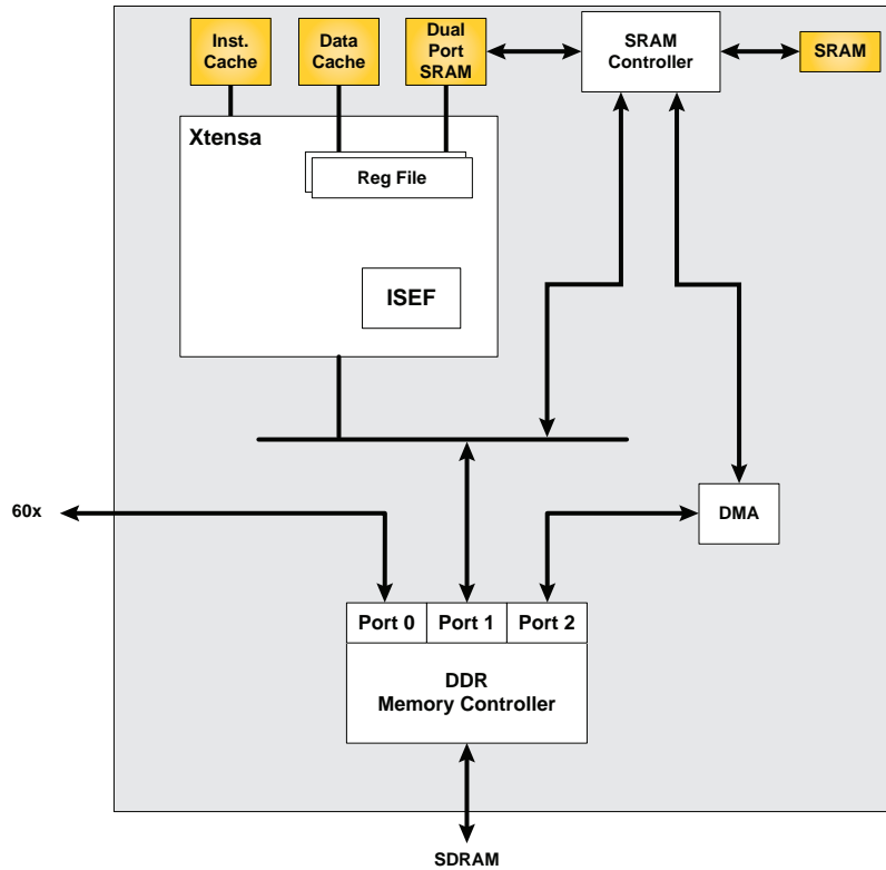
Figure 1-1 S5620 memory block diagram
