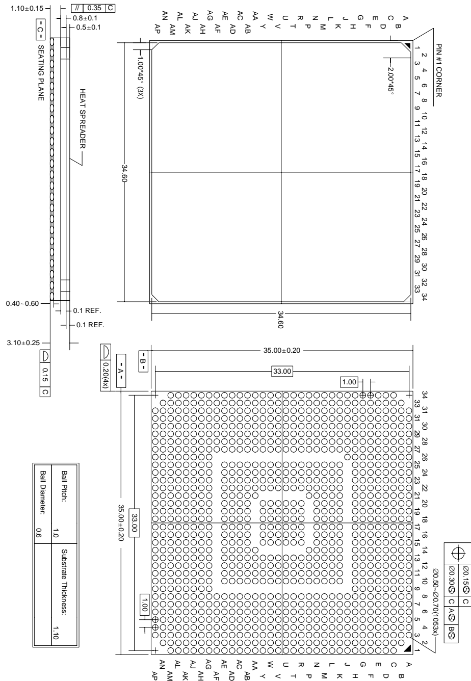
Figure 2-1 S5620 physical characteristics
