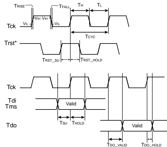
Figure 3-34 JTAG timing diagram
